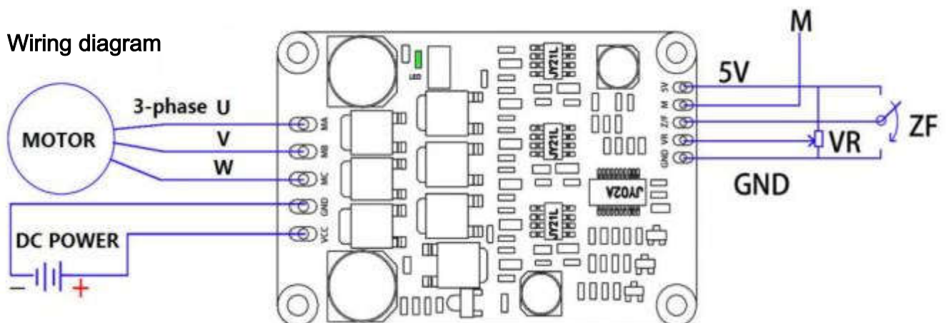
Driver board diagram
